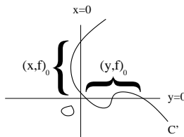
FIGURE 2. A Harnack smoothing of the cusp y^2 - x^3 = 0
