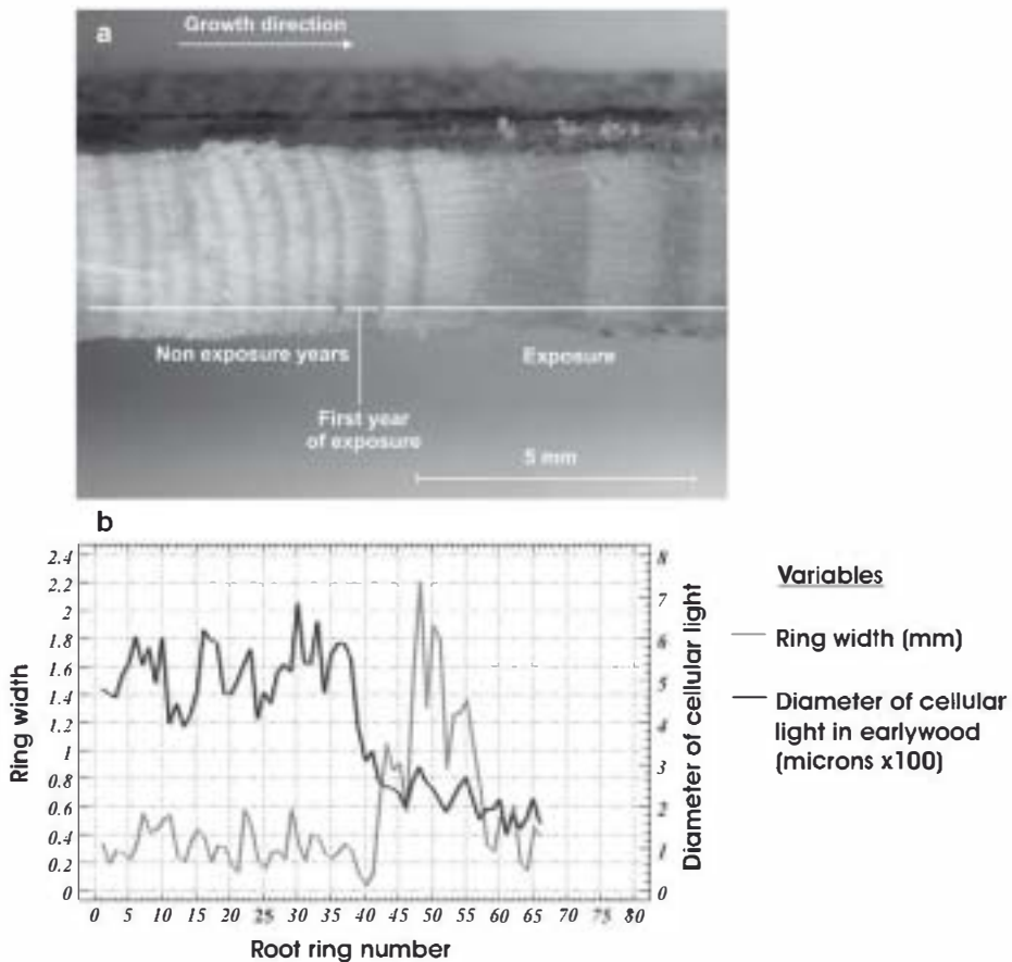
Fig. 4. (a) Change threshold in the ring-width measurement ( P. sylvestris , Senda Schmidt). The discontinuous line indicates the first year of exposure; (b) Variation in time in the tree ring-width series, as well as the diameter of cellular light in earlywood.
