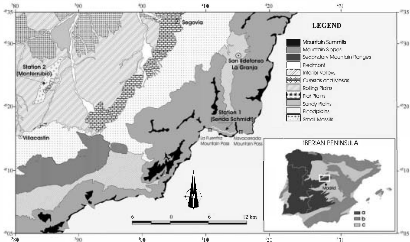
Fig. 1. Location of the two stations studied in the geomorphological context of the northern slope of the Sierra de Guadarrama, in the centre of the Iberian Peninsula: (a), Iberian Massif; (b) Alpine Belts; (c) Cenozoic Basins. The coordinates refer to zone 30T, Projection UTM, Hayford ellipsoid.
