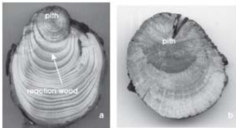
Fig. 3. Polished sections of the exposed roots of: (a) P. sylvestris , from Senda Schmidt. Note the eccentricity and presence of reaction wood after exposure. (b) Q. ilex , from the holm-oak forests in Montserriobio.
