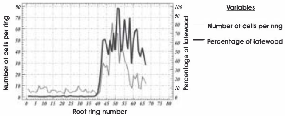
Fig. 5. Variation in the time of the number of cells per ring and of the latewood percentage ( P. sylvestris , Senda Schmidt).
