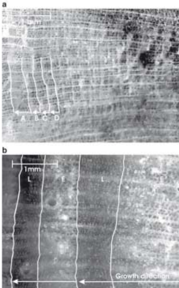
Fig. 6. (a) Cross-section of a P. sylvestris root in non-exposure conditions (A, B, C, D, represent growth rings). (b) Cross-section of a P. sylvestris root exposed by sheet erosion. Note the increasing growth ring width and the increasing percentage of latewood. L=latewood; E=earlywood.
