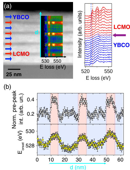
FIG. 2 (color online). (a) Z-contrast image of a LCMO/YBCO multilayer on a (100) \text{SrTiO}_3 substrate. Arrows mark LCMO (red) and YBCO layers (blue). The inset shows an EELS linescan acquired along the growth direction. The right panel shows the energy range corresponding to the O K edge across one of the YBCO-LCMO interfaces in the line scan. Dashed lines marked the position of the O prepeak for LCMO and YBCO away from the interface. (b) Prepeak intensity (top), and the edge onset position (bottom) along the growth direction, marked with a light blue arrow. Some data adapted from previous work (see Supplemental Material [33] for details)
