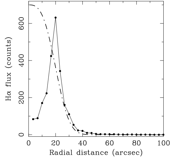
Fig. 7. H\alpha profile obtained using the isophotes measured in the R -band image ( solid-line ). The surface brightness profile of the plateau component as parametrized by Papaderos et al. (1996a) in the B -band is also shown ( dot-dashed-line ).
