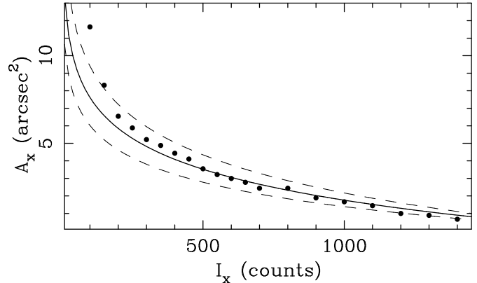
Fig. 11. Change in the area ( A_x ) of the region #18 with the threshold, I_x . The solid-line represents the result expected for a radius of 0''.9 at 1 e-folding. The dashed-lines correspond to 0''.8 and 1''.0 e-folding radii.
