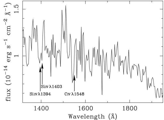
Fig. 4. IUE spectrum in the range 1150-1975Å obtained with the SWP camera in the low dispersion mode. The spectrum has been smoothed using a 2 pixels boxcar filter. The Si IV \lambda\lambda 1394,1403Å and C IV \lambda 1548Å spectral lines are shown with a clear P Cygni profile in the case of the C IV \lambda 1548Å line.
