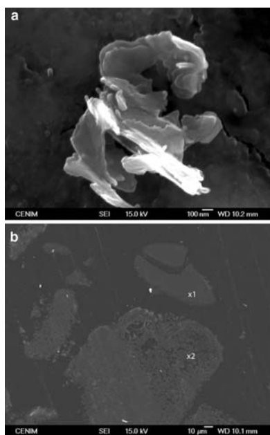
Fig. 3 SEM images a C12A7 crystal developed from nanoparticles aggregate obtained at pH 10 and 900 °C, b C2A (zone 1) and C12A7 (zone 2), obtained at pH 7 and 1100 °C
