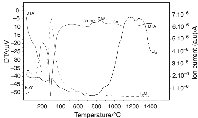
Fig. 6 DTA curve of sample obtained at pH 7 and curves of emission of \text{Cl}_2 and \text{H}_2\text{O} obtained by mass spectrometry
