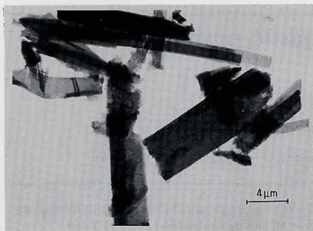
Figure 1 Electron micrograph of nickel hydroxychloride.
