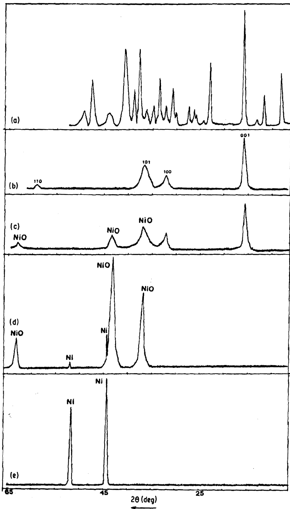
Figure 4 Evolution of nickel hydroxide when it is decomposed in the X-ray high-temperature diffraction chamber: (a) unheated; (b) 250°C ( a_{\text{hex}} = 0.317 nm, c_{\text{hex}} = 0.546 nm); (c) 400°C; (d) 680°C; (e) 720°C, 20 min.
