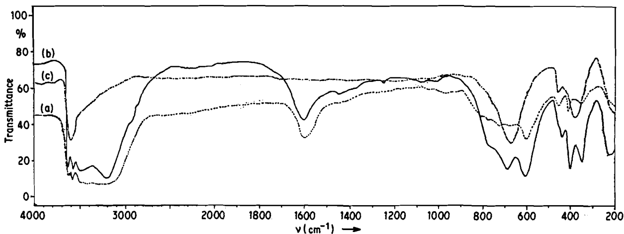
Figure 3 Infrared spectra of (a) (···) nickel hydroxychloride, (b) (—) heated at 180° C, (c) (-·-) heated at 280° C.
