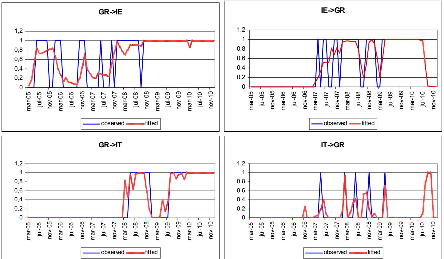
Figure 3: Probit results
