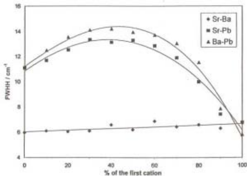
FIG. 3. (Top) Wavenumber of the sulfate anion symmetric stretching band against the chemical composition of the samples. (Bottom) Band full-width at half-height.
