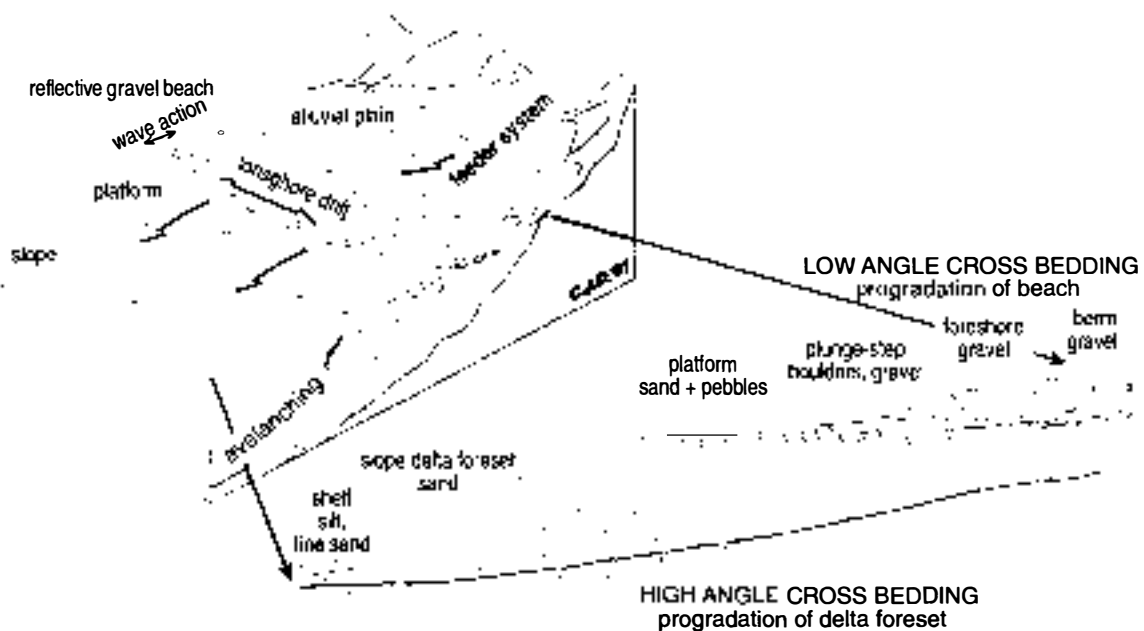
Fig. 8 - Model of Gilbert-type delta in Cuatro Calas (modified after Dabrio et al. , 1991).
