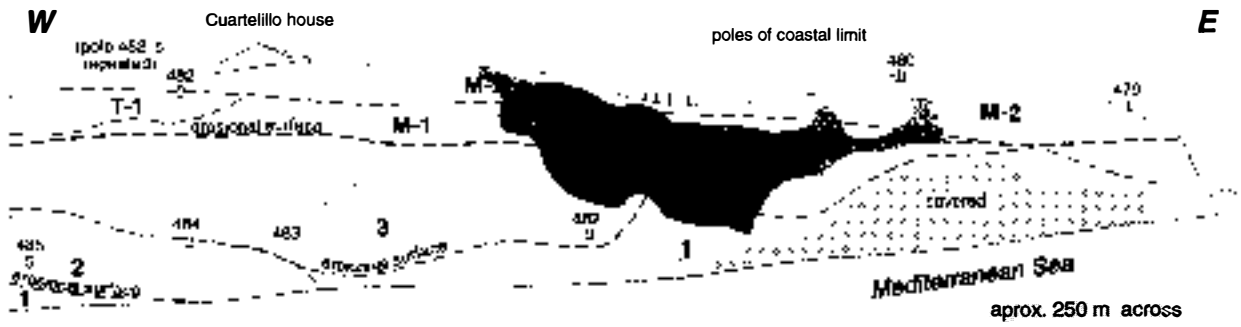
Fig. 7 - Panorama of the Cuartelillo hill (modified after Dabrio et al. , 1991). Numbers indicate sedimentary units.
