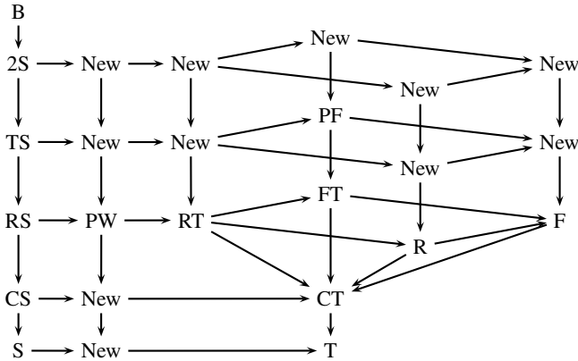
Fig. 3. The new linear time-branching time spectrum
