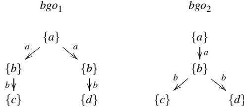
Fig. 1. Two branching observations
