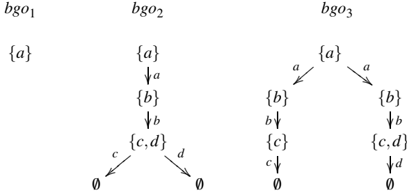
Fig. 2. Three branching observations
