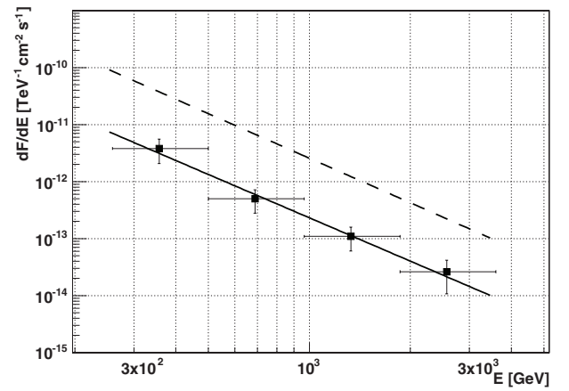
Figure 3. Spectrum of the complete LS I +61°303 data sample recorded by the MAGIC stereo system in 2009 is shown in black. The vertical errors are 1\sigma statistical errors. The fit to the most precise measured spectrum from Fall 2006 (Albert et al. 2009) is shown as the dashed line. The 2009 spectrum is fitted by a simple power law as well and the fit parameters are compatible to our previous measurements from 2005 to 2008 (see the text for discussion).
