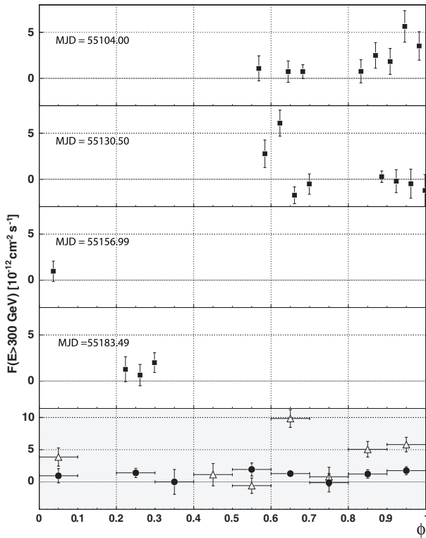
Figure 2. VHE ( E > 300 GeV) \gamma -ray flux of LS I +61°303 as a function of the orbital phase for the four observed orbital cycles (four upper panels) and averaged for the entire observation time (lowermost panel, black points). The starting MJD of each orbital cycle is given in the corresponding panel. In the lower most panel we show as hollow triangles the previous published (Anderhub et al. 2009) averaged fluxes per phase bin. Vertical error bars show 1\sigma statistical errors.
