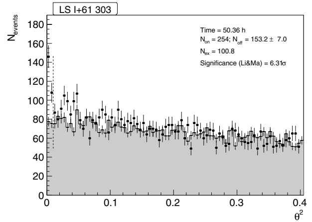
Figure 1. Squared angular distance between the pointing direction of the shower and the source position ( \theta^2 -plot) for the position of LS I +61°303 (points) and the simultaneous determined background regions (gray shaded histogram) for the total 2009/2010 MAGIC data set. N_{\text{on}} is the number of events at the source position, N_{\text{off}} is the number of background events, N_{\text{ex}} is the number of excess events ( N_{\text{ex}} = N_{\text{on}} - N_{\text{off}} ), and the significance was calculated according to Li & Ma (1983).
