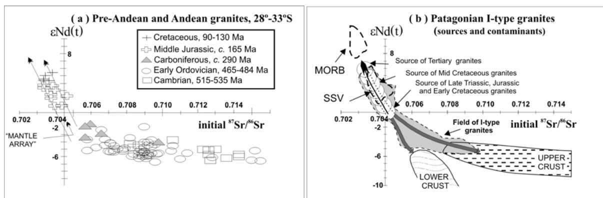
Figure 3. Variation of \epsilon\text{Nd}_t versus initial ^{87}\text{Sr}/^{86}\text{Sr} for the granitic rocks emplaced during the main convergence episodes in the Andean sector at 28°- 33°S (a) and Patagonia (b). Data sources are Pankhurst et al. , 1999; 2000, Parada et al. , 1999, Rapela et al. , 2005, Hervé et al. , 2007 and references therein.
