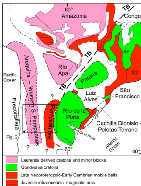
Figure 1. Group of cratons and minor blocks amalgamated in the Pampean-Araguaia orogeny (540-515 Ma) (modified from Trindade et al. , 2006 and Rapela et al. , 2007). TB = Transbrasiliano shear zone.
