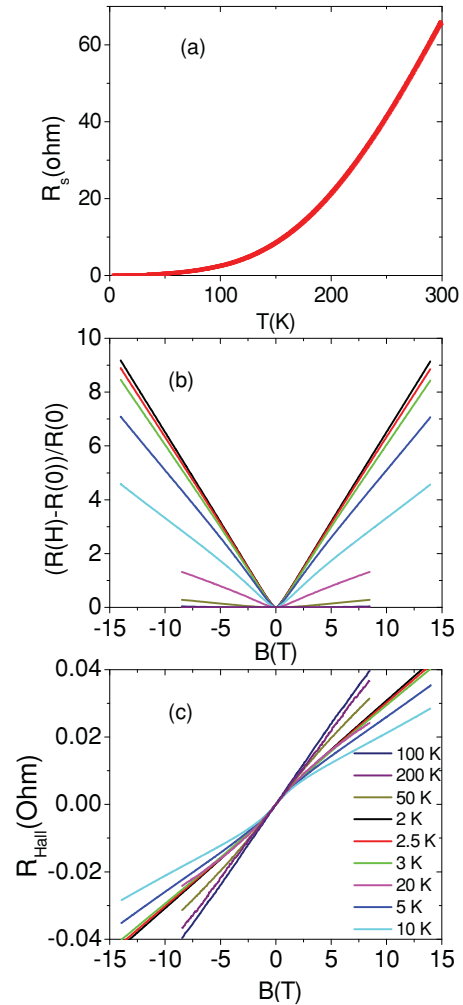
FIG. 1. (Color online) (a) Temperature dependence of the sheet resistance in zero applied magnetic field of STO crystals irradiated at a power of 30 W for 5 min. Magnetic field dependence of the 4 probe (van der Pauw) magnetoresistance at 200, 100, 50, 20, 10, 5, 3, 2.5 and 2 K (from bottom to top) (b) and Hall effect at 100, 200, 50, 2, 2.5, 3, 20, 5, and 10 (from bottom to top at 8 T) (c) in magnetic fields applied perpendicular to the crystal surface.
