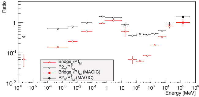
Fig. 3. P2_M/P1_M ratio (black markers) and \text{Bridge}_E/P1_M ratio (red markers) as a function of energy. At optical energies (a few eV), the ratios are obtained using the central pixel of the MAGIC camera (Lucarelli et al. 2008). From 100 eV to 100 MeV, ratios are computed based on the light curves shown in Kuiper et al. (2001). From 100 MeV to 30 GeV, Fermi -LAT data were used.
