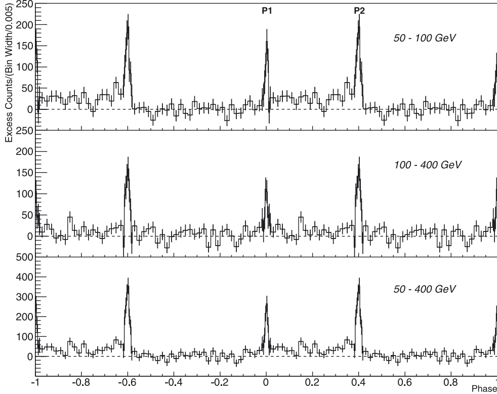
Fig. 1. Light curves of the Crab pulsar obtained by MAGIC from 50 GeV to 100 GeV ( top ), from 100 GeV to 400 GeV ( middle ), and for the full analyzed energy range ( bottom ). The bin widths around the peaks are 4 times smaller (0.005) than the rest (0.02) in order to highlight the sharpness of the peaks.
