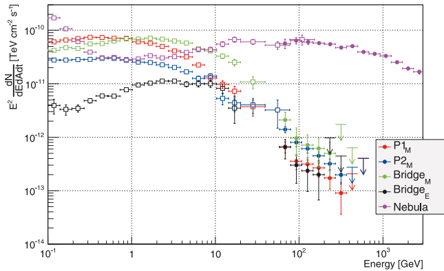
Fig. 4. Spectral energy distributions of the Crab nebula, P1_M , P2_M , \text{Bridge}_M , and \text{Bridge}_E measured with Fermi -LAT (below 50 GeV) and MAGIC (above 50 GeV). The flux values averaged over the rotation period are plotted.
