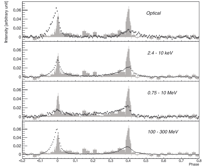
Fig. 2. Light curve of the Crab pulsar at optical wavelength, 2.4–10 keV X-rays, 0.75–10 MeV, and 100–300 MeV gamma rays ( from top to bottom ). The light curve at 50–400 GeV is overlaid on each plot for comparison. The optical light curve was obtained with the MAGIC telescope using the central pixel of the camera (Lucarelli et al. 2008). The keV and MeV light curves are from Kuiper et al. (2001). The 100–300 MeV light curve was produced using the Fermi -LAT data. All light curves are zero-suppressed by estimating the background using the events in the phase range from 0.52 to 0.87.
