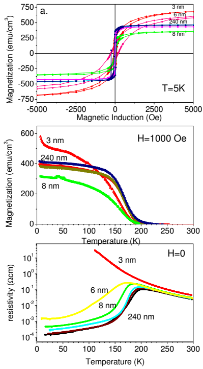
Fig. 1 (a) Magnetization hysteresis loops, (b) temperature dependent magnetisation (c) and resistivity of LCMO thin films with various thicknesses between 3 and 240 nm.
