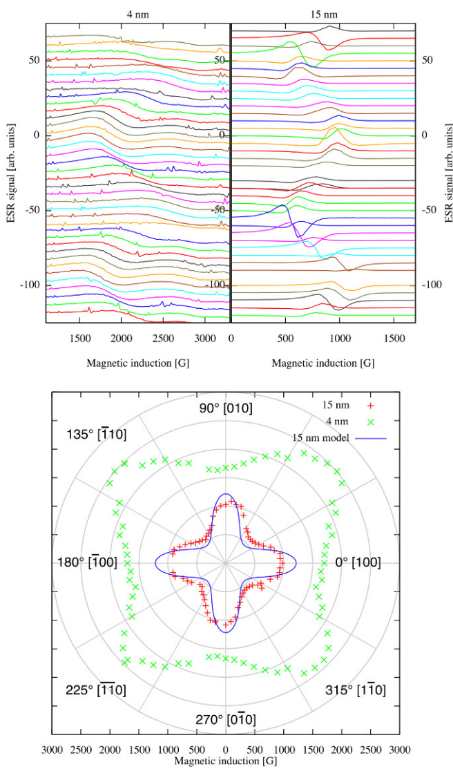
Fig. 3 (top) Ferromagnetic resonance spectra at f=8.88 GHz in d=4 nm (left) and d=15 nm (right) LCMO thin films at 77 K with the external magnetic field lying along various in-plane directions. The spectra were linearly displaced so that their baseline position indicates the in-plane angle. (bottom) FMR positions shown in polar-plot for both 4 and 15 nm thin films. The blue curve is a model for the 15 nm sample as described in the text. The radial axis corresponds to the magnetic field from 0 to 3000 G. Some of the 4 nm points are not independent data but mirrored from equivalent positions.
