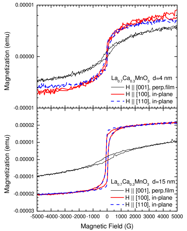
Fig. 2 Magnetization hysteresis loops of d=4\text{ nm} (top) and d=15\text{ nm} (bottom) LCMO thin films with the external magnetic field lying along [100] and [110] in-plane directions and along [001], perpendicular to the film-plane, at 77 K.
