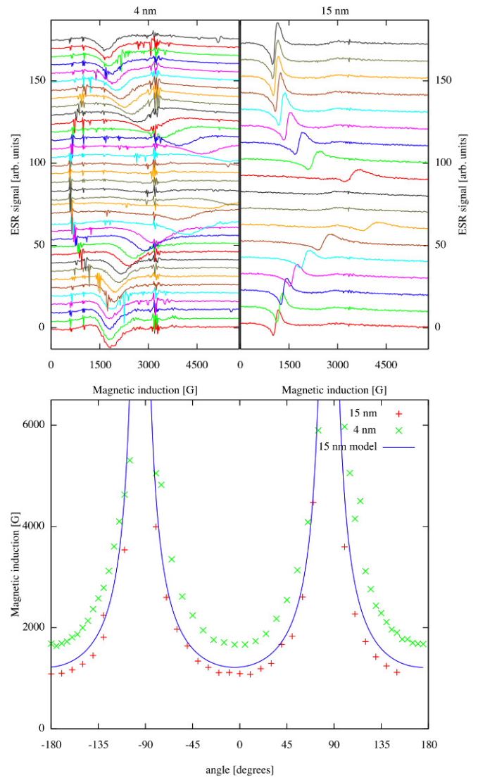
Fig. 4 (top) Ferromagnetic resonance spectra at f=8.88 GHz in d=4 nm (left) and d=15 nm (right) LCMO thin films with the external magnetic field rotated out-of-plane. The spectra were linearly displaced so that their baseline position indicates the out-of-plane angle, 90 being the field perpendicular to plane configuration. (bottom) FMR positions for both 4 and 15 nm thin films. The blue curve is a model for the 15 nm sample as described in the text.
