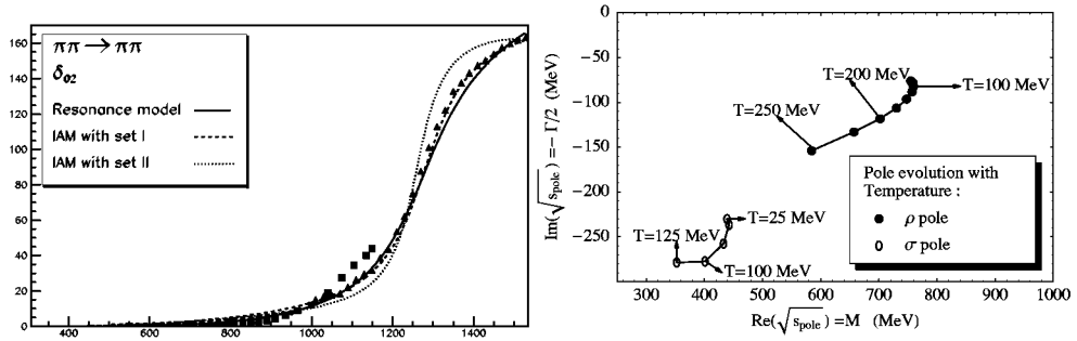
FIGURE 2. a) The I=0, J=2 \pi\pi scattering phase shift [15] and the results of our unitarized chiral resonance model (continuous line), of eq.(6) with the parameters in set I (dashed line), and with those in set II (dotted line) in Table 3. b) Thermal evolution of the \sigma and \rho poles.
