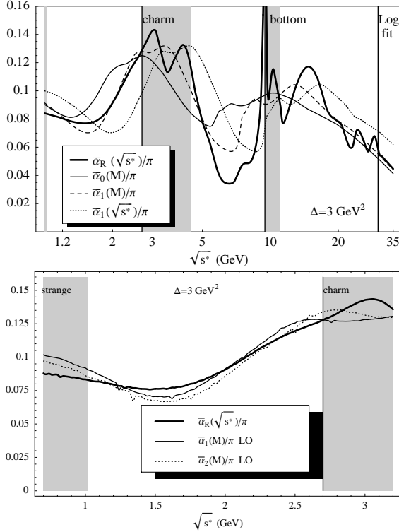
Figure 2.a) Comparison between \bar{\alpha}_R(\sqrt{s^*}) and different \bar{\alpha}_k moments at M = \sqrt{s^*}/\lambda_k . The dotted line shows how the agreement is spoiled if we do not shift \sqrt{s^*} to M . b) Comparison between \bar{\alpha}_R(\sqrt{s^*}) and different \bar{\alpha}_k moments at M = \sqrt{s^*}/\lambda_k in the low energy region.
