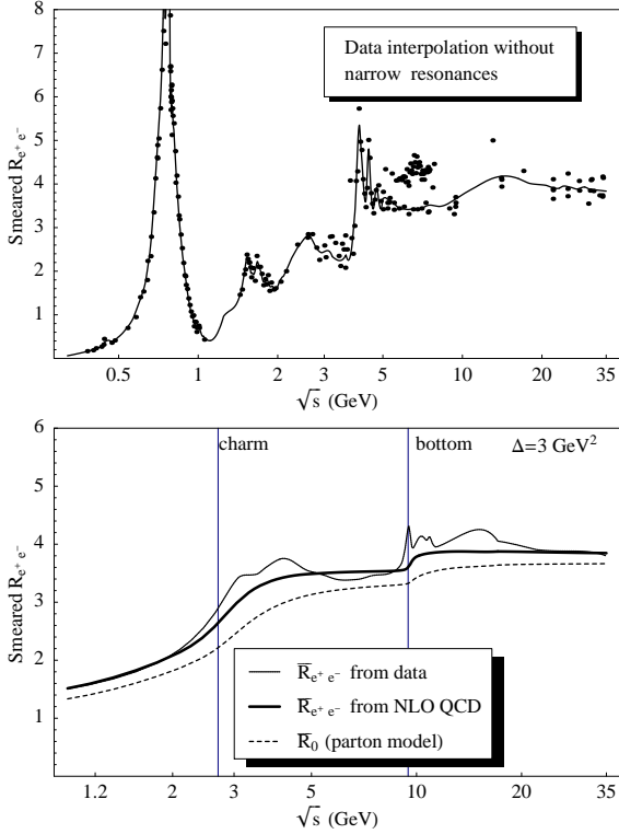
Figure 1.a) Interpolation of the central values of R_{e^+e^-} -data (see [3] for references). Note the discrepancy in the central values of experiments between 5 and 10 GeV. b) Smeared R_{e^+e^-} .
