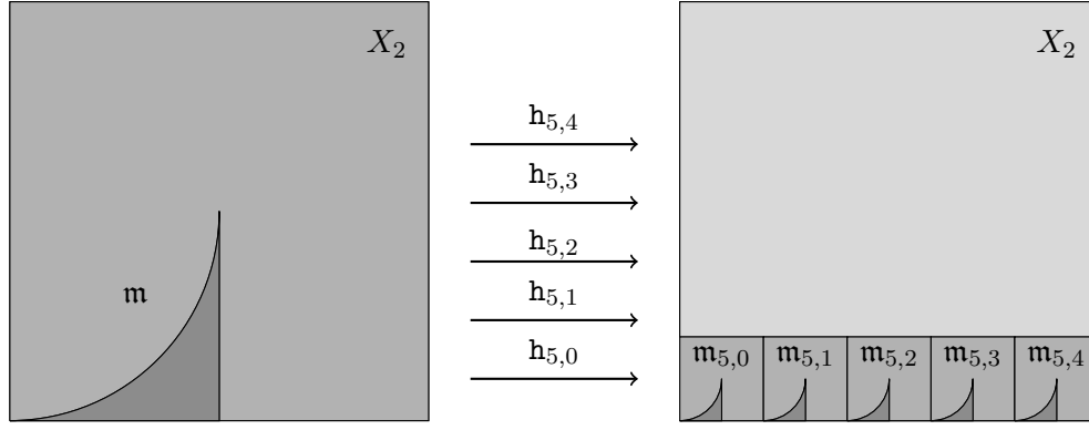
FIGURE 1. Construction of the maximal ideals \mathfrak{m}_{k,\ell} for m = 2 (and k = 5 ).
