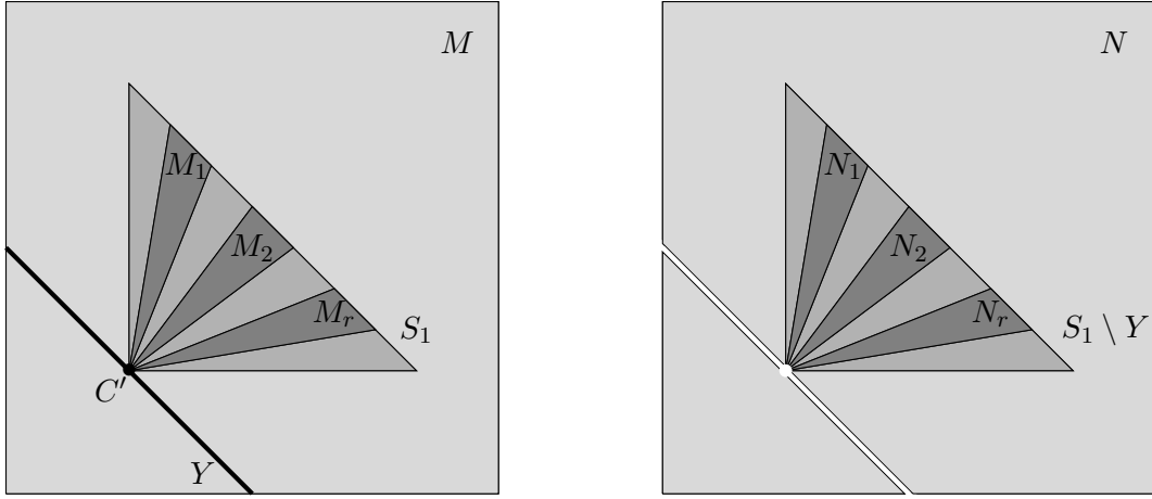
FIGURE 3. Construction of the semialgebraic sets M_i and N_i .
