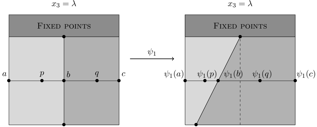
FIGURE 2. Restriction of the map \psi_1 to the plane x_3 = \lambda for m = 3 .
