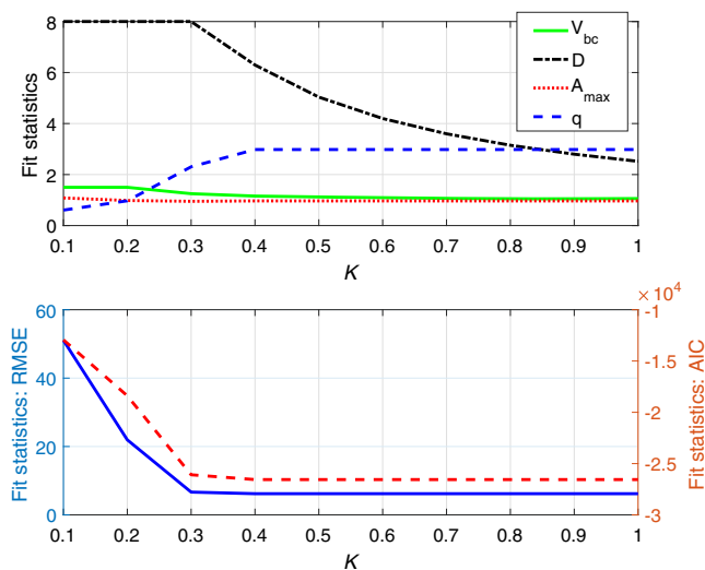
Fig. 4 In the upper plot, we show the evolution of the values of the fitting parameters V_{bc} (continuous line, green in color), pupil diameter (dash-dotted black line), maximum accommodation (dotted line, red in color), diameter (dash-dot line, black in color), and parameter q (dashed line, blue in color). In the lower plot, we have represented the fit statistics RMSE (left vertical axis, blue in color) and AIC (right vertical axis, red in color) against K parameter when fitting Peters's data to our model.
