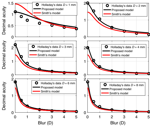
Fig. 2 Model fit to the complete set of data given by Holladay et al. (circles). We have represented the V against blur for different pupil sizes; the dark curves (black in color) are the results obtained after applying our model using the coefficients of MAR_H(D) with the parameters obtained through the fit shown in Fig. 1. The light (red in color) curves represents the results obtained after fitting the modified Smith's model proposed in Eq. (12) to the same data set.
