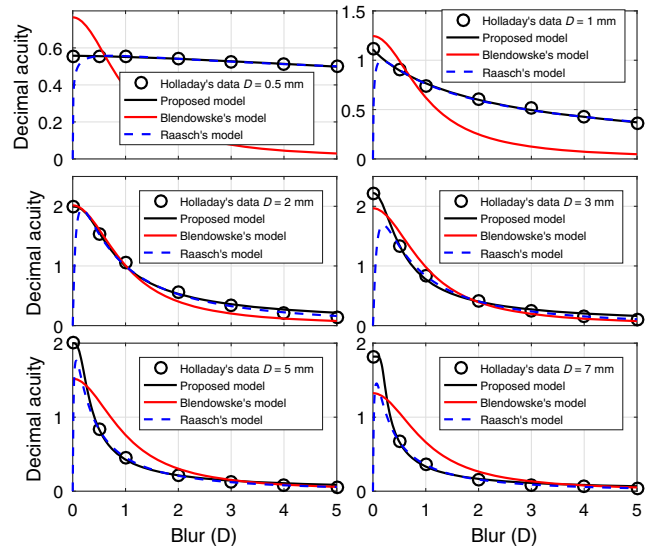
Fig. 3 Model fit to the complete set of data given by Holladay et al. (circles) taken pupil by pupil so that each panel represents the fit of the models to the values of Holladay et al.'s V corresponding only to this pupil diameter. We have represented the V against blur for different pupil sizes; the dark curves (black in color) are the results obtained after applying our model using the coefficients of MAR_H(D) with the parameters obtained through the fit shown in Fig. 1. The light (red in color) curves represents the results obtained after fitting Blendowske's model, and the dashed curves (blue in color) represent the fitting of the data to Raasch's model.
