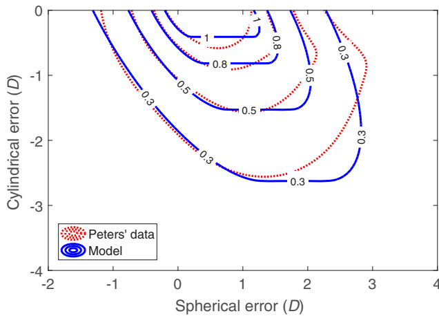
Fig. 5 Contour plot of visual acuity against spherical and cylindrical error. The dashed line represents the values given by Peters for the group of individuals whose age was between 45 and 55 years old (group III in Ref. 10) while the solid line represents the direct fitting of the proposed model to those data.
