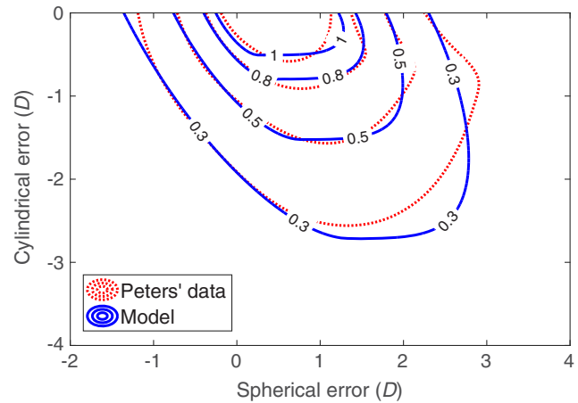
Fig. 6 Contour plot of visual acuity against spherical and cylindrical error. The dashed line represents the values given by Peters for the group of individuals whose age was between 45- and 55-years old (group III in Ref. 10) while the solid line represents the fitting of those data to the proposed model following the statistical averaging procedure described in the text.
