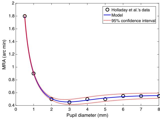
Fig. 1 Best corrected (zero blur) MAR as a function of pupil diameter as given by Holladay et al. (circles), and fit of these data to the model function MAR_H(D) plotted as a continuous line (blue in color). The 95% confidence interval of the model is also plotted as two dashed lines (red in color).
