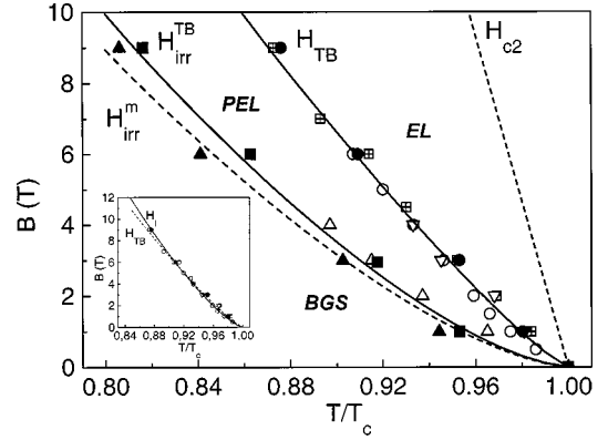
FIG. 7. Magnetic phase diagram of the liquid vortex state of Y123/211 melt-textured composites for H_{\parallel c} . Indicated are: ( \blacktriangle ) the intrinsic irreversibility line, H_{\text{irr}}^m(T) , obtained from the anisotropic Ginzburg-Landau model, ( \blacksquare ) the quenched Bose glass transition line due to twin boundary pinning, H_{\text{irr}}^{\text{TB}}(T) , and ( \bullet ) the H_{\text{TB}}(T) transition indicating the transition from a partially entangled liquid to a fully entangled liquid. Also shown are the Bose glass transition for ( \triangle ) a twinned single crystal, the H_{\text{TB}}(T) line for ( \circ ) a twinned Y123 single crystal and the H^*(T) line for ( \boxplus ) a Y123/211 melt-textured composite and ( \nabla ) a twinned single crystal both obtained from flux transformer experiments. The mean field H_{c2}(T) and the regions indicating the Bose glass solid (BGS), partially entangled liquid (PEL), or disentangled liquid (DL) for the case of single crystals and, the entangled liquid (EL) phases, are also represented. In the inset, all four H_{\text{TB}}(T) data sets are again shown and compared to the fit to the scaling law H_1/|t|^{2\nu} = \text{const} with \nu = 0.699 suggested by Nguyen and Sudbo (Ref. 21) and the best fit H_{\text{TB}}(T) = 105(1 - T_{\text{TB}}/T_c)^{1.2} shown in their Fig. 7.
