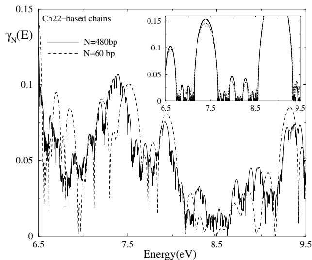
FIG. 4. Lyapunov coefficient for Ch22-based (main frame) and Fibonacci Polygc quasiperiodic-based sequences for the same number of bp (inset).
