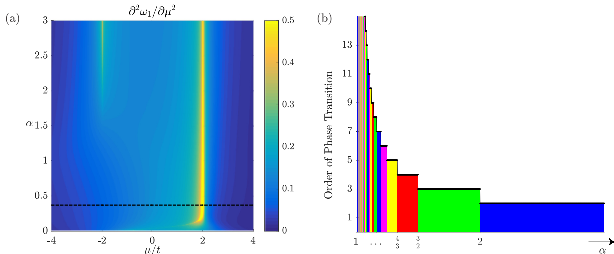
FIG. 1. (a) Second derivative of the bulk thermodynamic potential, obtained from Eq. (5) for the LRKC on the \mu/t - \alpha plane. The dashed line indicates the value of \alpha below which our numerical results are not accurate anymore. (b) Staircase of higher-order topological phase transition at \mu/t = -2 , indicating how the order of the transition increases as one approaches \alpha = 1 .
