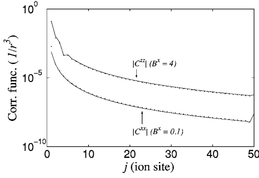
FIG. 7. (a) Absolute value of correlations |C_{j_0 j_0+j}^{\alpha\alpha}| ( j_0=50 , N=100 ions) in the case of the 1/r^3 Ising model. Points, numerical results from the DMRG calculations; solid line, calculation with the HP transformation.
