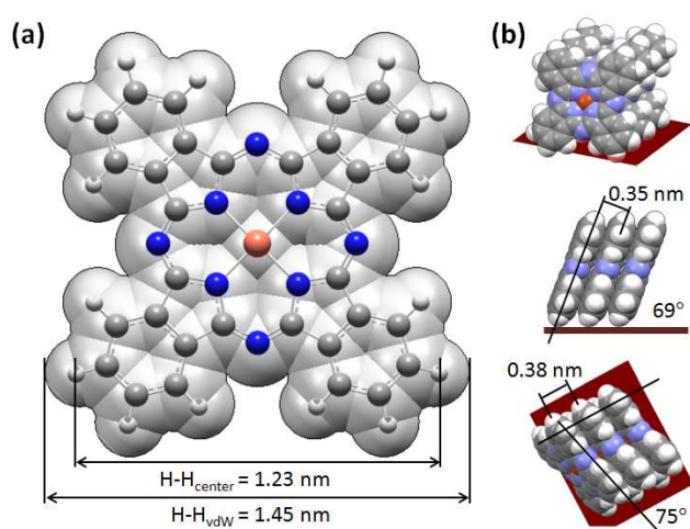
Fig. 1 (a) Chemical structure of a copper(II) phthalocyanine (CuPc) molecule as resulting from DFT calculations; the corresponding van der Waals (vdW) overlapping sphere model is shown in the background. (b) Molecular stack geometry as determined from single crystal x-ray diffraction 10 . Intra-stack periodicity (0.38 nm), \pi - \pi stacking distance (0.35 nm), and inclinations of the molecular planes against the stacking direction are indicated.
