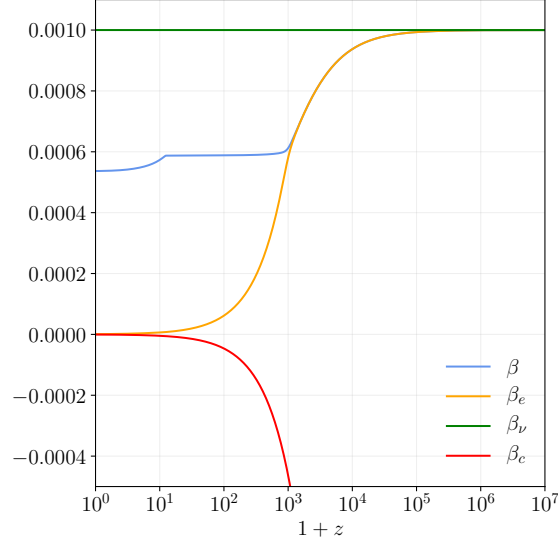
FIG. 1: Time evolution of the bulk velocities for the different components. The dark matter velocity is obtained enforcing the cosmic center of mass condition (151). Massless neutrinos behave as an uncoupled ultrarelativistic species throughout the evolution and maintain a constant velocity. The photon-baryon plasma behaves as a single fluid, either matter- or radiation-like, until decoupling z_{\text{dec}} \simeq 1090 . Around z \simeq 11 there is a small effect in the photon velocity due to reionization.
