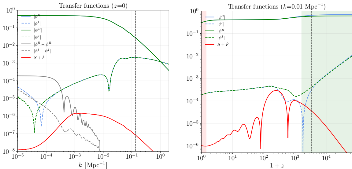
FIG. 5: Transfer functions, with initial curvature perturbation normalized to one, in the Newtonian gauge. Both panels represent the evolution of the Newtonian potentials, their difference and the vector metric perturbation. The imaginary parts and the vector modes are proportional to \beta_0 . We show the results for \beta_0 = 10^{-3} . (Left) The vertical line indicates the super-Hubble and non-linearity scales, respectively. The sharp drop in the difference between the Newtonian potentials at small scales is a consequence of the RSA. On those scales we are setting the shear of ultrarelativistic species to zero, since it has a negligible impact in our observables. (Right) The vertical line marks the horizon crossing. In the red and green shaded regions the RSA and TCA, respectively, are switched on.
