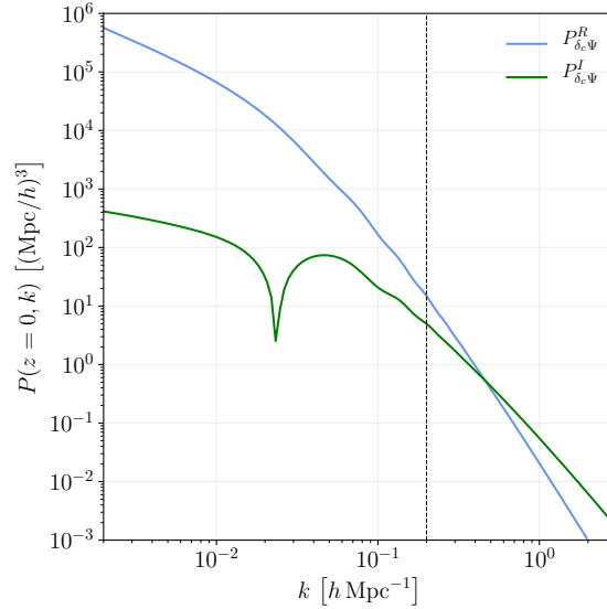
FIG. 7: The vertical line indicates the scale of non-linearity. Cross-correlation spectra of dark matter density and lensing potential \Psi \equiv \phi + \psi , including both the standard and the dipolar contribution. P_{\delta_c \Psi}^I is given in units (\beta_0/10^{-3})(\text{Mpc}/h)^3 .
