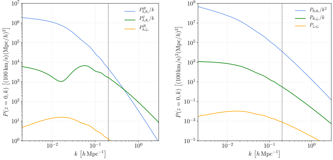
FIG. 6: The vertical line indicates the scale of non-linearity. (Left) Cross-correlation spectra of dark matter densities and velocities, including the standard as well as the dipolar contribution, both for the divergence and for the vorticity. P_{\delta_c \theta_c}^I and P_{\delta_c \zeta_c}^R are given in units of (\beta_0/10^{-3})(100 \text{ km/s})(\text{Mpc}/h)^3 , i.e. the curves are plotted for \beta_0 = 10^{-3} but the spectra are proportional to this value. (Right) Autocorrelation spectra of dark matter velocity, as well as the cross-correlation spectrum between vorticity and the divergence of the velocity. P_{\theta_c \zeta_c} and P_{\zeta_c \zeta_c}^R are given in units (\beta_0/10^{-3})(100 \text{ km/s})^2(\text{Mpc}/h)^3 and (\beta_0/10^{-3})^2(100 \text{ km/s})^2(\text{Mpc}/h)^3 , respectively.
