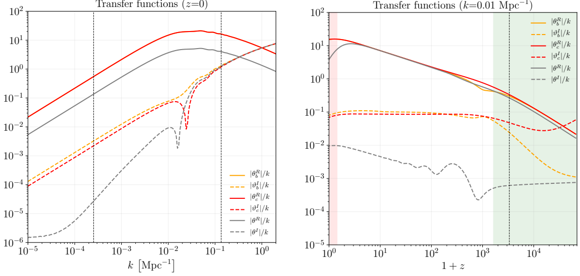
FIG. 3: Transfer functions, with initial curvature perturbation normalized to one, in the Newtonian gauge. Both panels represent the evolution of the velocity divergence, where the imaginary parts have been redefined according to (247). The imaginary parts are proportional to \beta_0 . We show the results for \beta_0 = 10^{-3} . (Left) The vertical line indicates the super-Hubble and non-linearity scales, respectively. (Right) The vertical line marks the horizon crossing. In the red and green shaded regions the RSA and TCA, respectively, are switched on.
