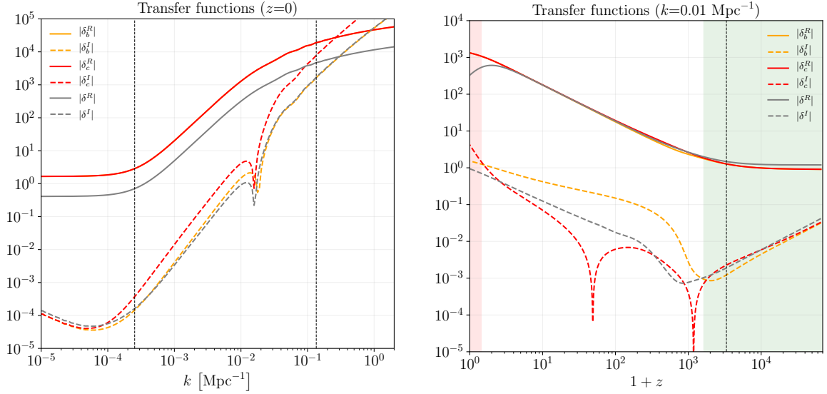
FIG. 2: Transfer functions, with initial curvature perturbation normalized to one, in the Newtonian gauge. Both panels represent the evolution of the density contrast, both the standard and our modification. The imaginary parts are proportional to \beta_0 . We show the results for \beta_0 = 10^{-3} . (Left) The vertical line indicates the super-Hubble and non-linearity scales, respectively. (Right) The vertical line marks the horizon crossing. In the red and green shaded regions the RSA and TCA, respectively, are switched on.
