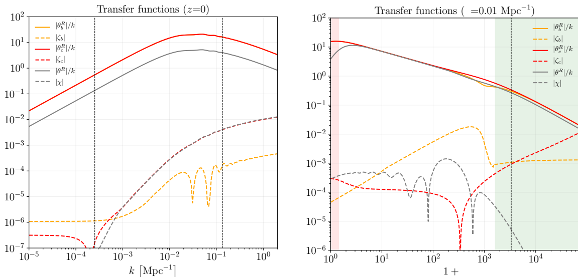
FIG. 4: Transfer functions, with initial curvature perturbation normalized to one, in the Newtonian gauge. Both panels represent the evolution of the vorticity, compared with the velocity divergence. Again, the vorticity has been redefined according to (247). The vorticity is proportional to \beta_0 . We show the results for \beta_0 = 10^{-3} . (Left) The vertical line indicates the super-Hubble and non-linearity scales, respectively. (Right) The vertical line marks the horizon crossing. In the red and green shaded regions the RSA and TCA, respectively, are switched on.
