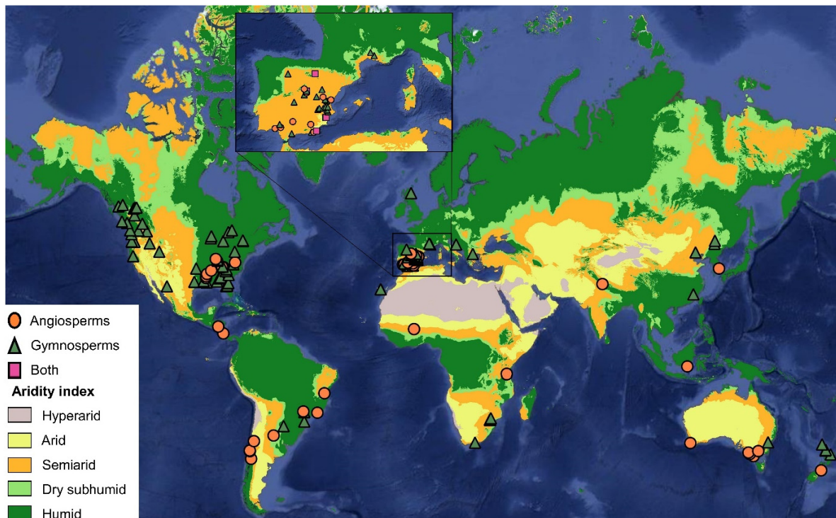
FIG. 1. Distribution of planting locations ( n = 142 ) from studies used in the meta-analysis with indication if planted species are angiosperms or gymnosperms. Different colors on the map indicate regions with the same climatic classification according to the global aridity index.
