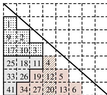
FIGURE 4.6. Lattice representation of the gap set \mathbb{N} \setminus \Gamma .
