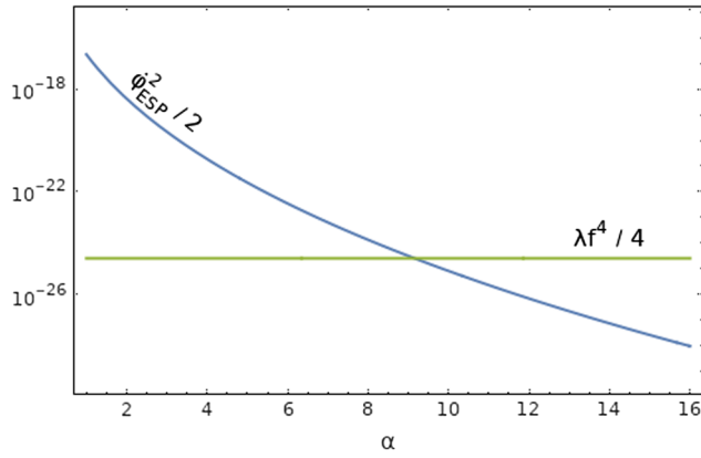
FIG. 2. The inflaton kinetic energy density at ESP (blue curve) and the false vacuum energy density (green line) as a function of \alpha . In this plot we used the best fit value of n_s (within 2\sigma range the result depends mildly on the precise value of n_s ) and we took \lambda = 1 and f = 10^{12} GeV.
