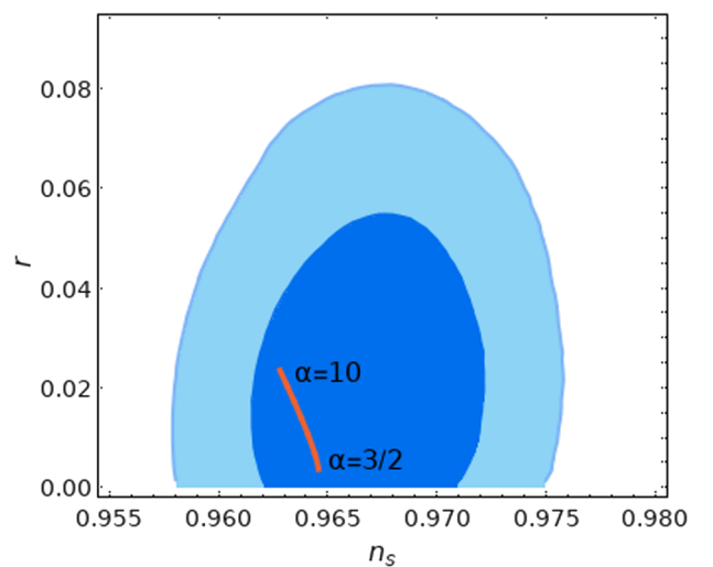
FIG. 4. The 1\sigma and 2\sigma contours of the Planck constraints from Ref. [38]. The red curve is the prediction of our model assuming Eq. (73).
