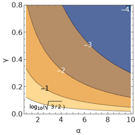
FIG. 3. A contour plot of \log_{10}(\Phi_1/m_{\text{Pl}}) values as a function of \alpha and \gamma [see Eq. (59)]. In this plot we used \lambda f^2/\gamma\dot{\varphi}_{\text{ESP}} \ll 2/3^{3/2} and the best fit value n_s = 0.968 . The plot changes insignificantly within the allowed 2\sigma range of n_s . The white region is where the condition in Eq. (58) is violated, i.e., where the expansion of the Universe cannot be neglected.
