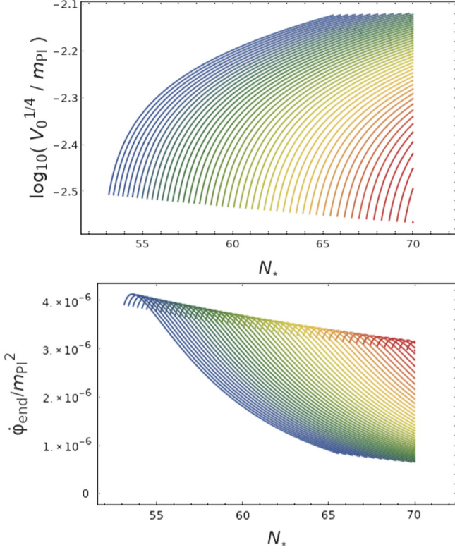
FIG. 1. The allowed range of V_0 values (upper) and the field velocity at the end of inflation \dot{\phi}_{\text{end}} (lower) as a function of N_* . Each curve represents a fixed value of the scalar spectral index n_s . The blue leftmost curve is for the 2\sigma lower bound n_s = 0.962 and the red rightmost curve is for n_s = 0.971 . We used the central value \ln(10^{10}A_s) = 3.094 of the spectrum normalization in Eq. (25).
