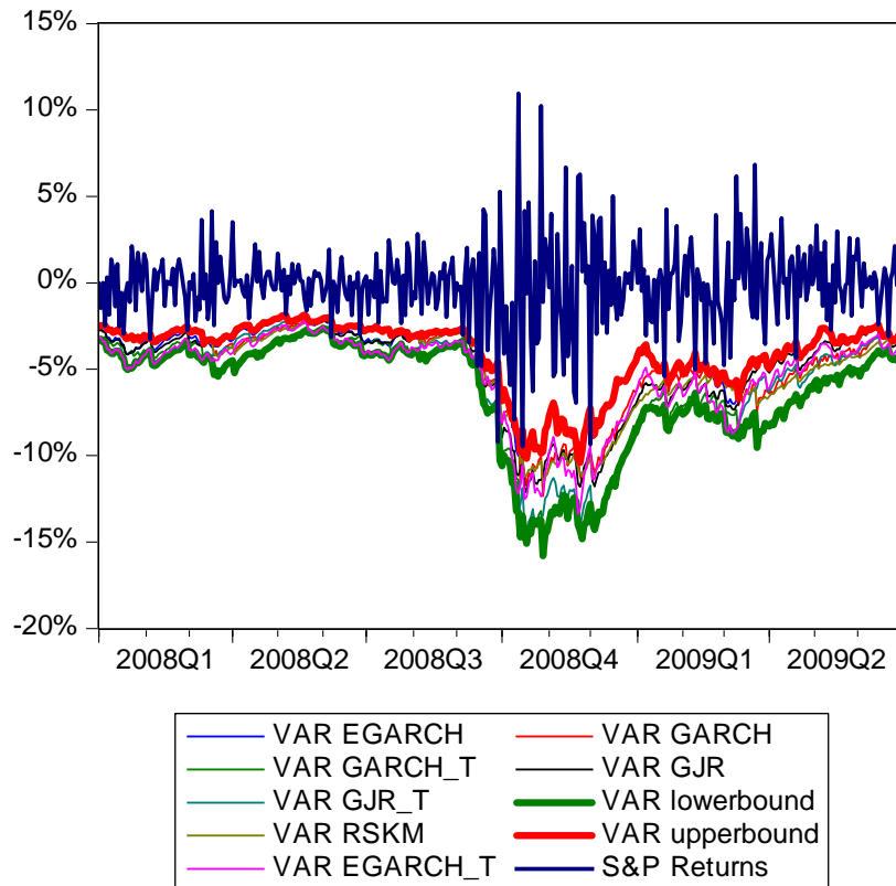
Figure 4. VaR for S&P500 Returns, 2 January, 2008 –2 July, 2009
